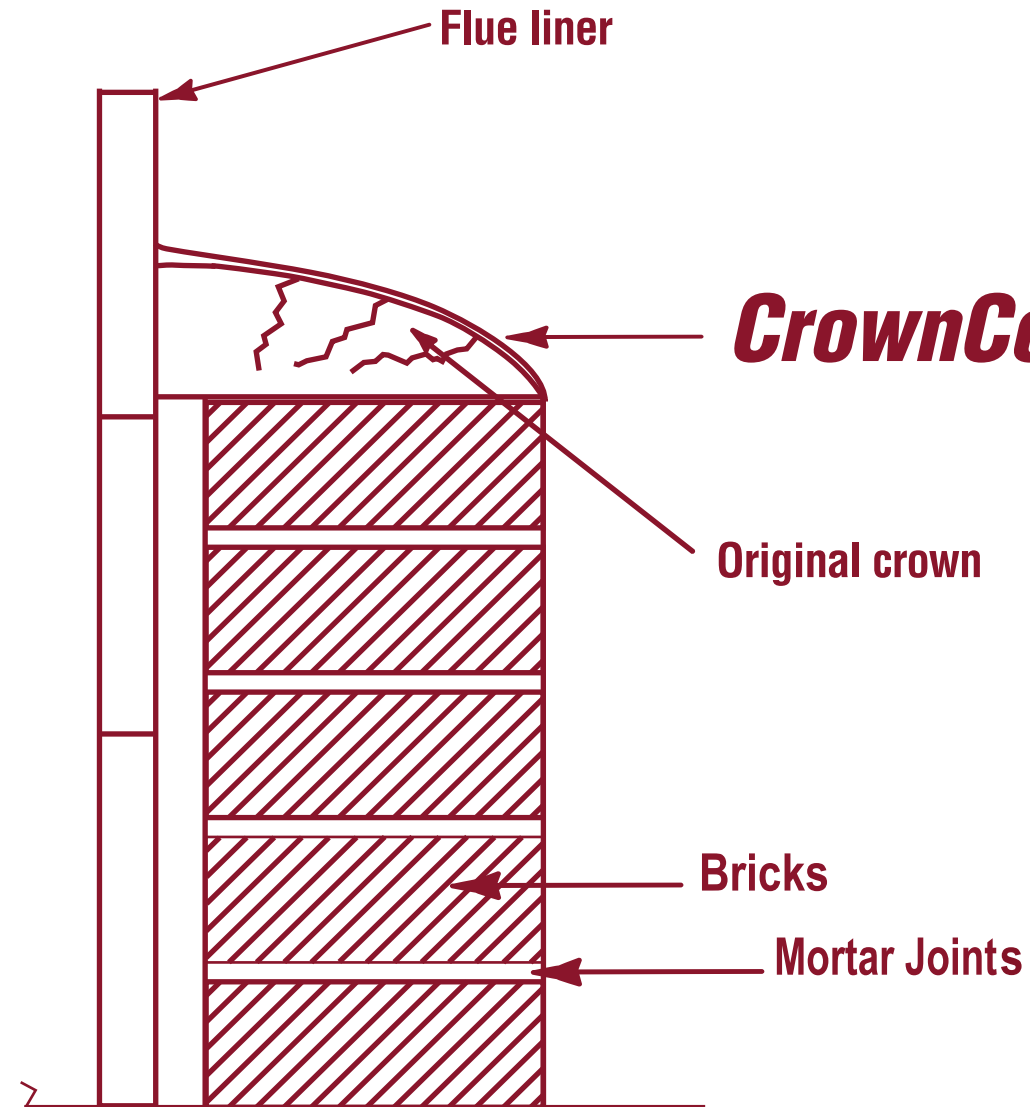
Side View of Masonry Chimney
